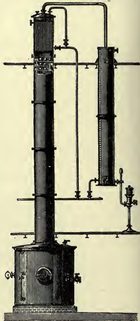
FIG. 4.—Benzol Still (elevation), scale \frac{1}{4} .
